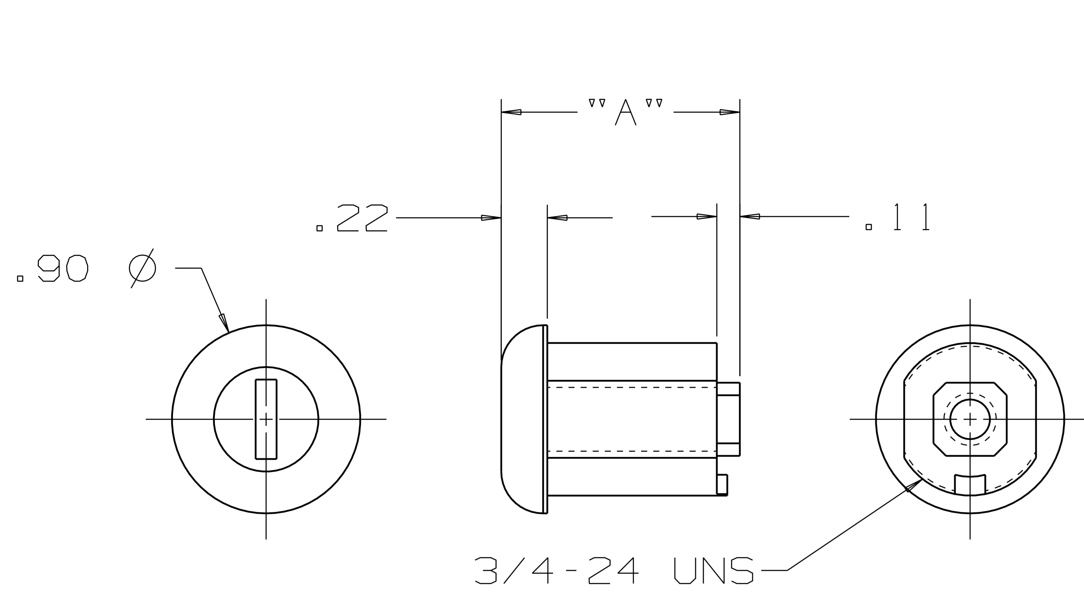
LOCK ASSY
