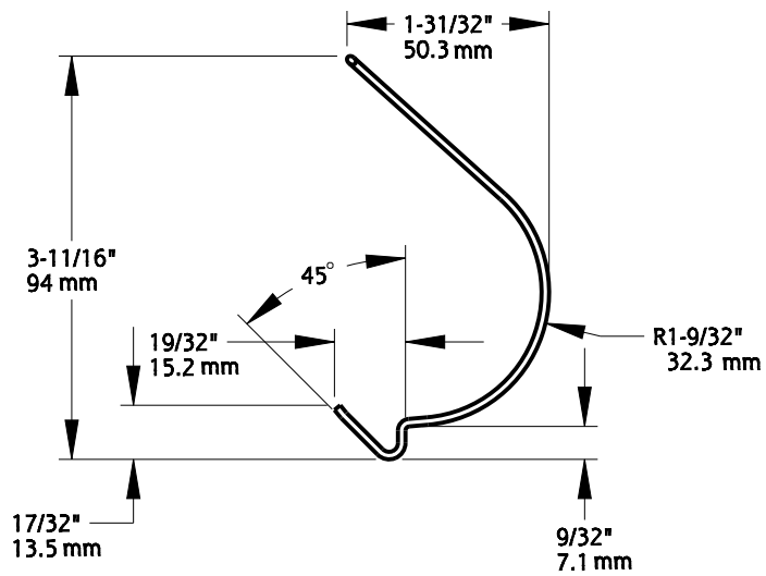
LIGHT J-HOOK WIRE: \phi 0.070" [ \phi 1.78mm] SWL: 10 POUNDS IN 1/2" DRYWALL
